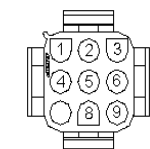
CHASSIS HARNESS CONNECTOR (C1) (MATING SIDE)
