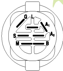
IGNITION SWITCH
