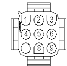
CHASSIS HARNESS CONNECTOR (C1) (MATING SIDE)
