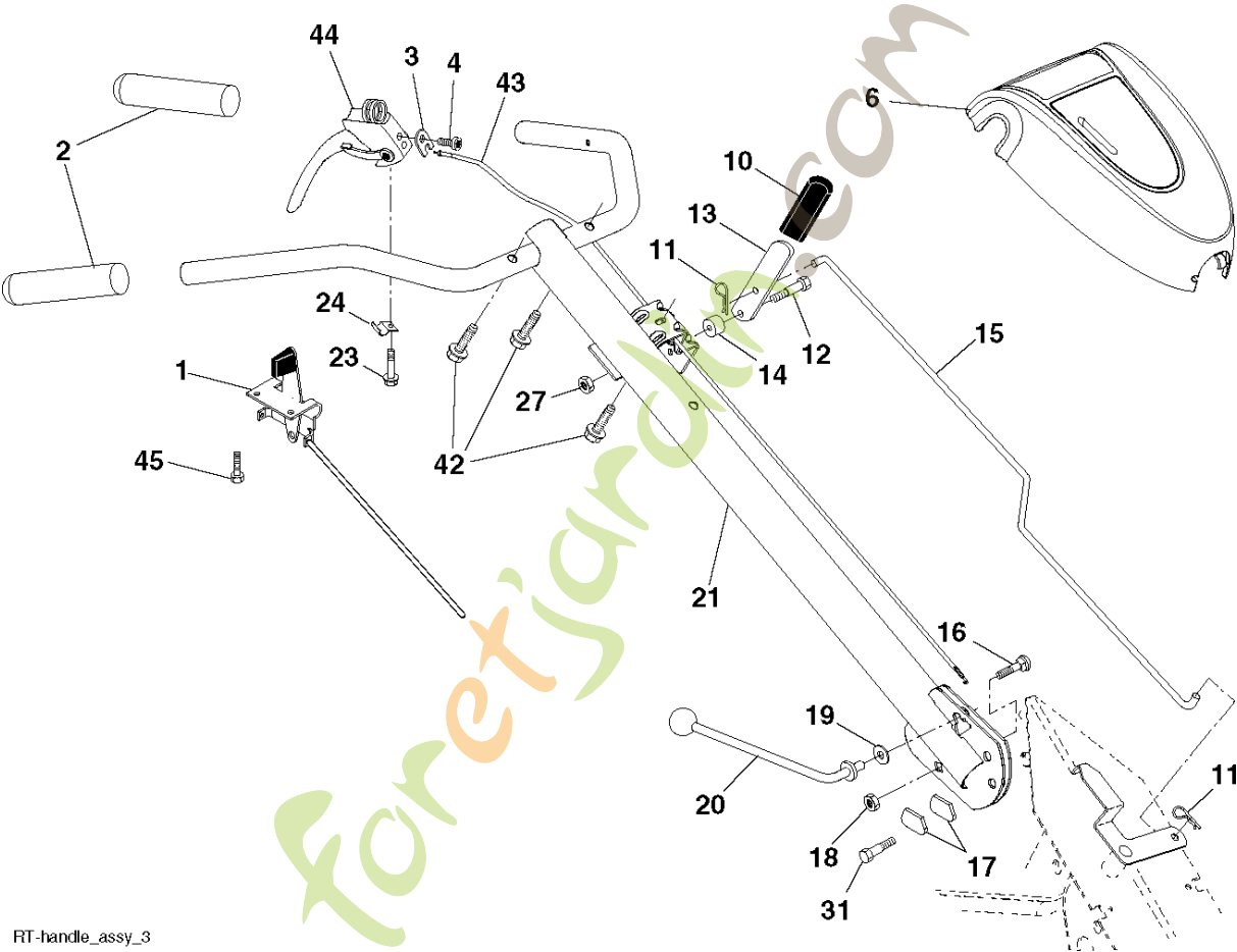
RT-handle_assy_3
