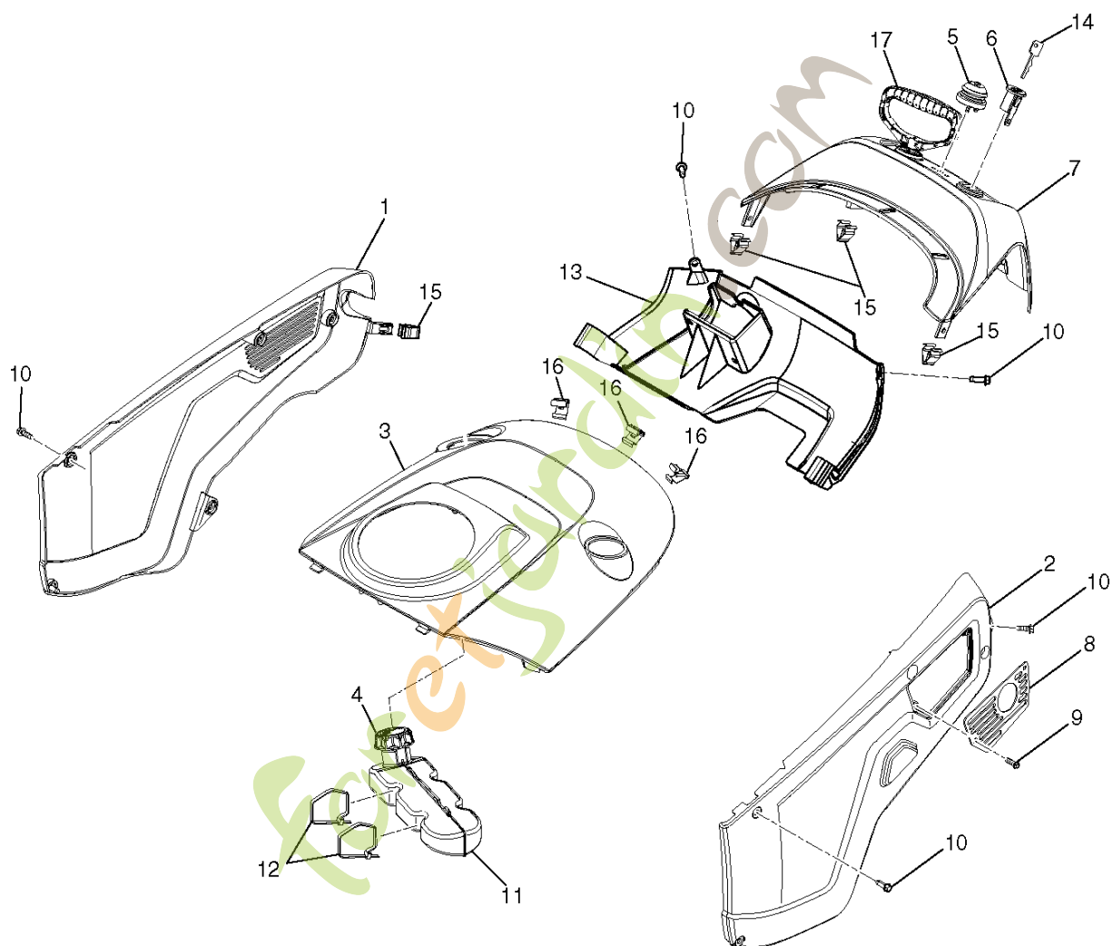
SSST-Shroud asm_17
