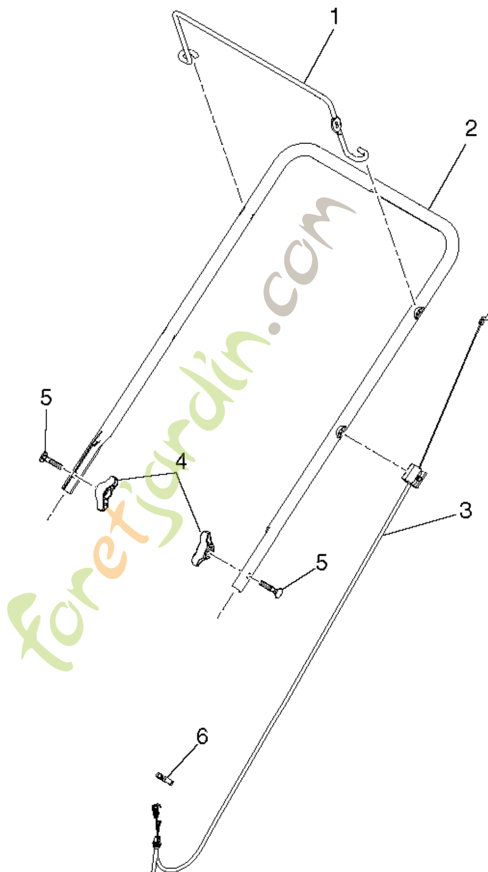
SSST-Handle asm_1
