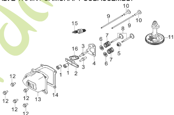
E05 VALVE TRAIN / CAMSHAFT SUBASSEMBLY
