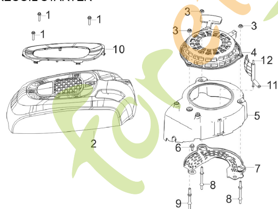
E06 RECOIL STARTER
