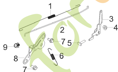
E13 THROTTLE CONTROL ASSEMBLY
