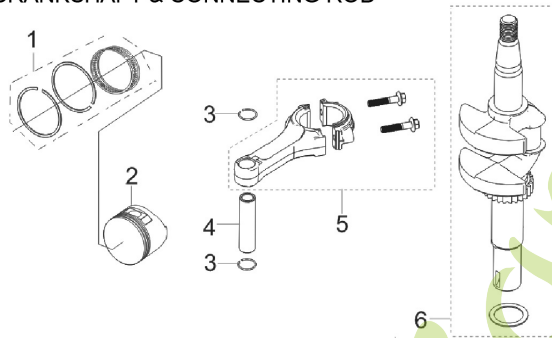
E04 CRANKSHAFT & CONNECTING ROD
