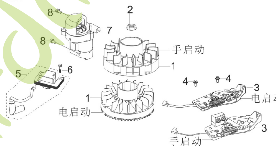
E12 FLYWHEEL, IMPELLER, STARTER PULLEY, IGNITION COIL
