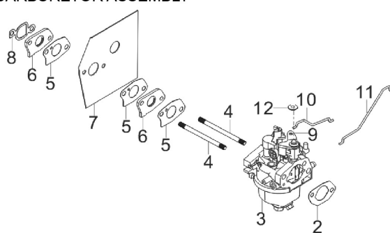
E08 CARBURETOR ASSEMBLY
