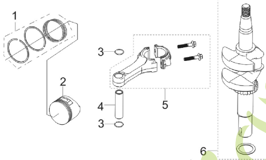
E04 CRANKSHAFT & CONNECTING ROD
