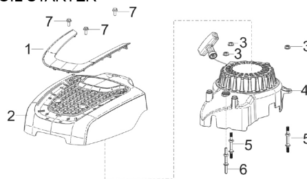
E06 RECOIL STARTER
