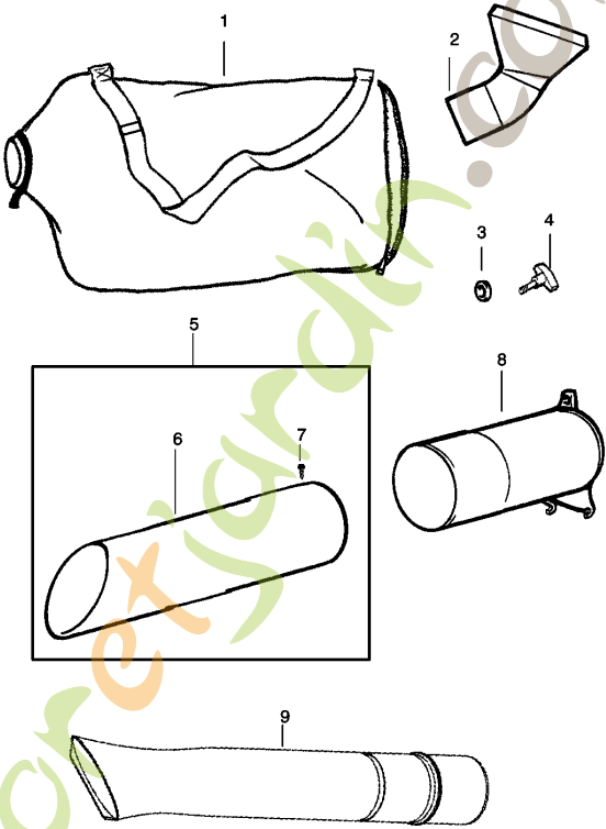
Assy - Vacuum
