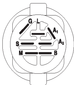
IGNITION SWITCH
