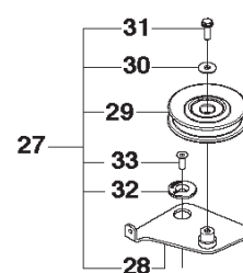
Large bushing
